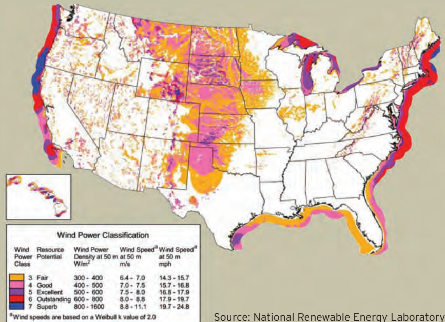
FIGURE 3: UNITED STATES OFFSHORE WIND RESOURCE
